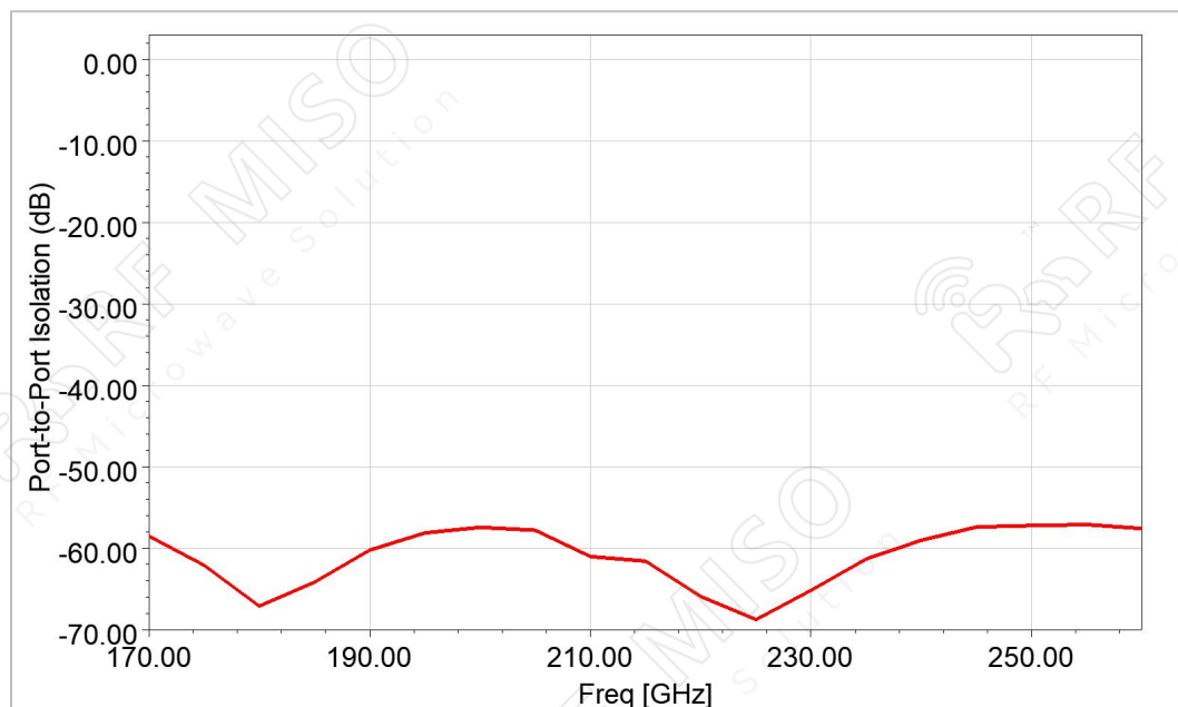
Isolation
