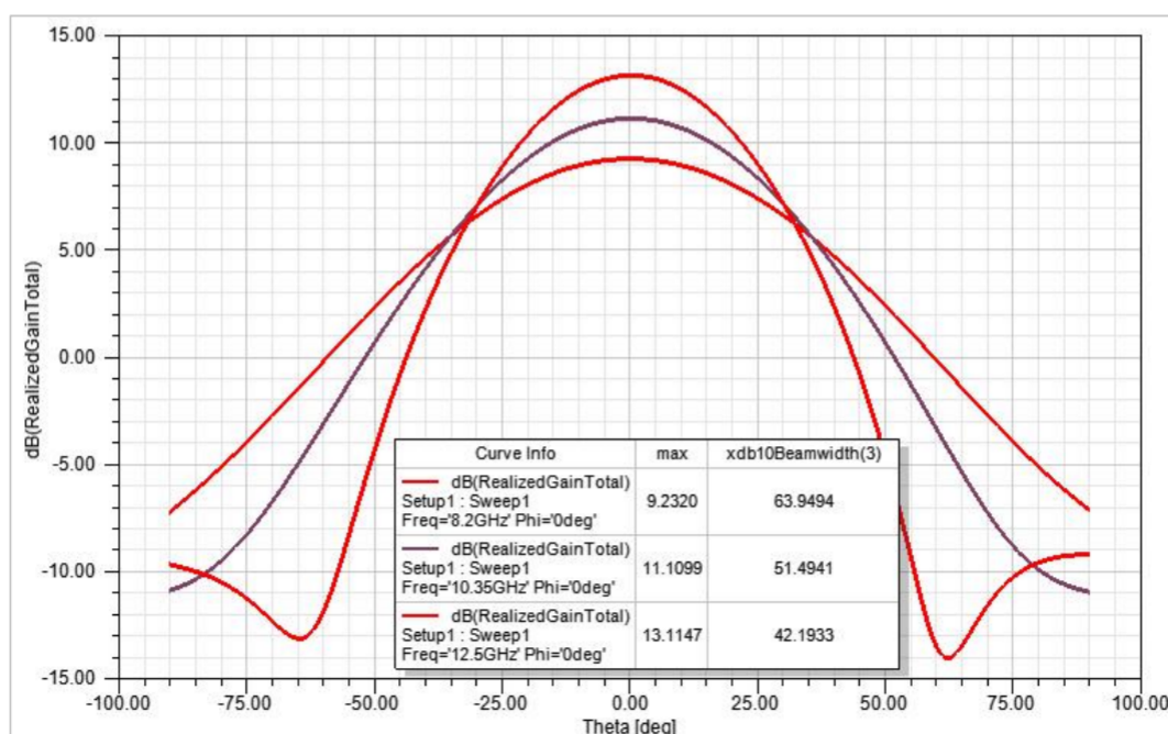
Gain Pattern E-plane
