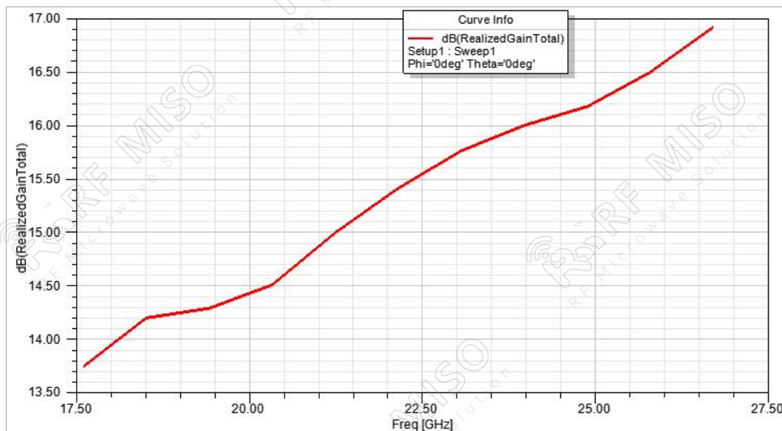
Gain
