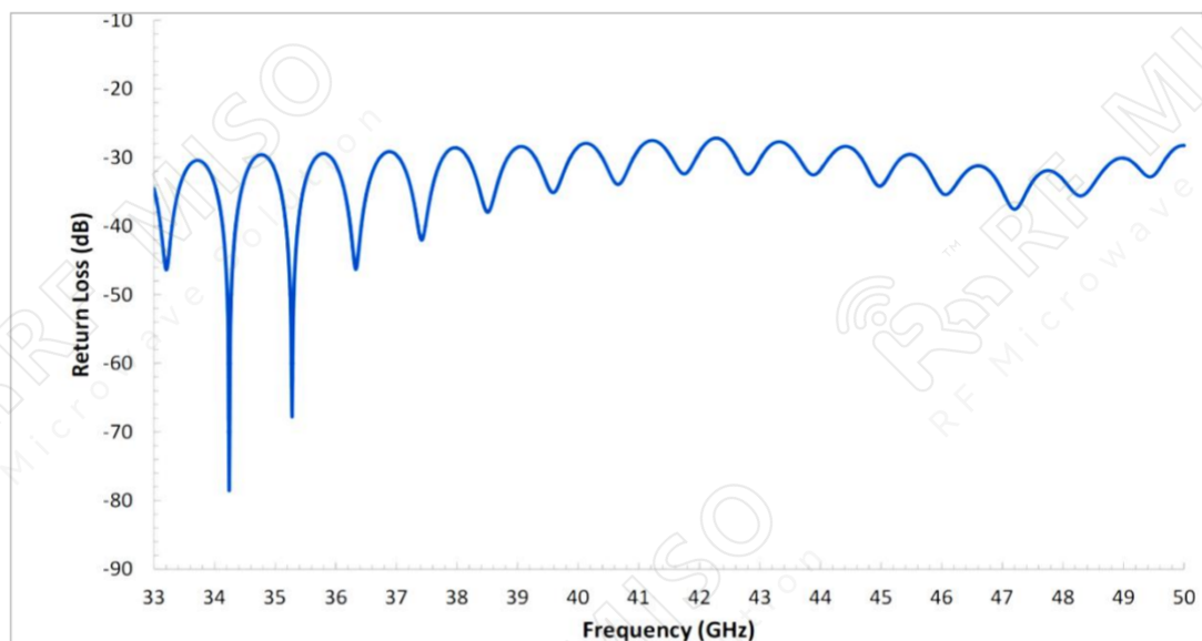
Return Loss
