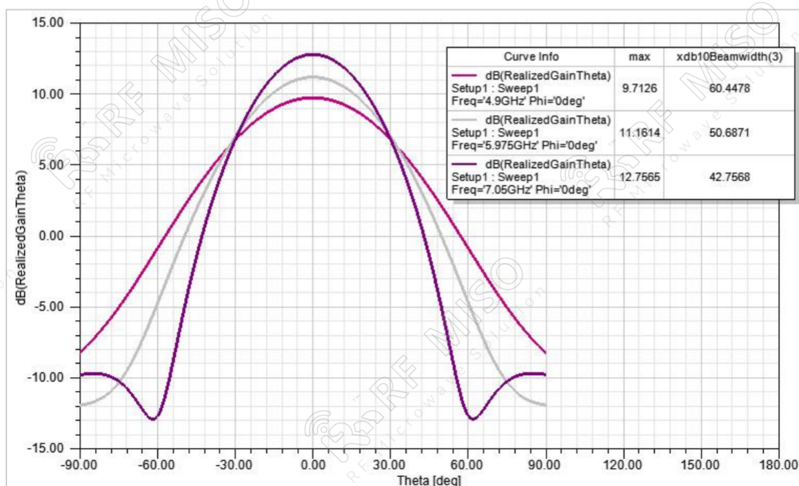
Gain Pattern E-plane
