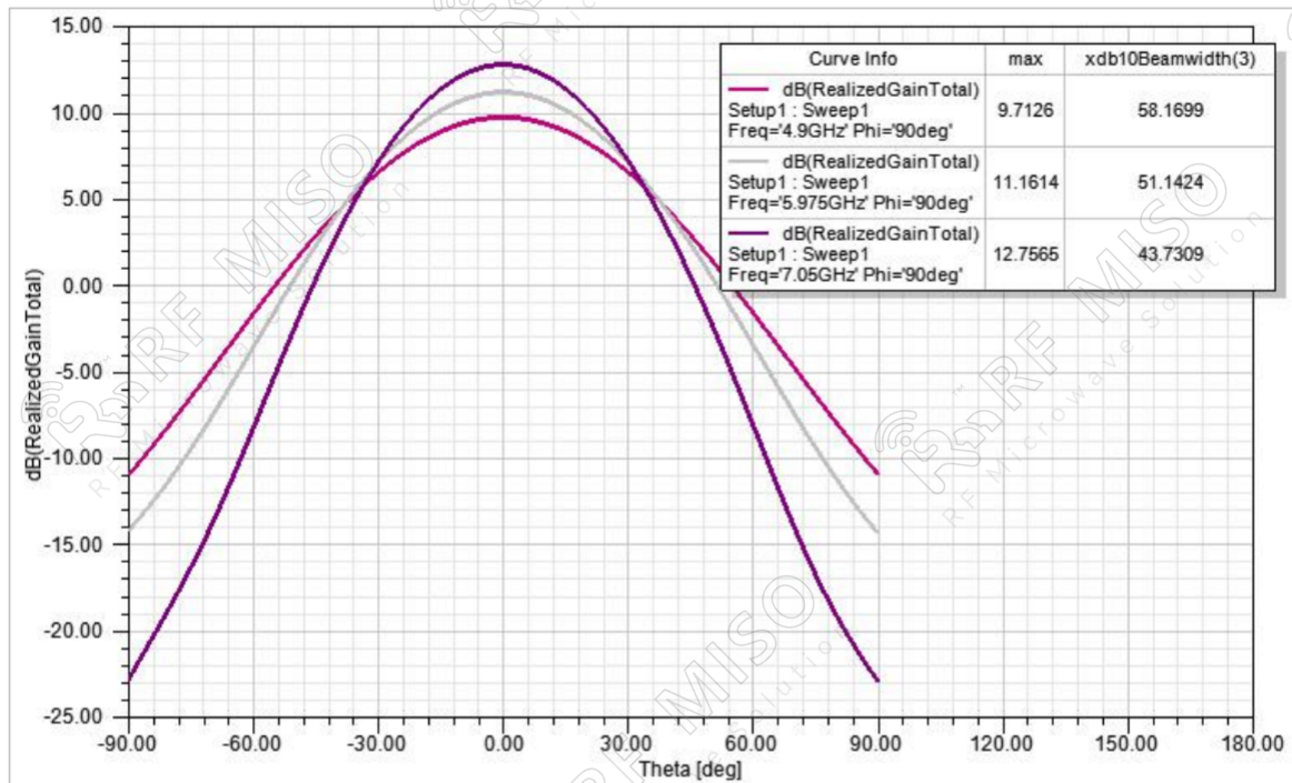
Gain Pattern H-plane
