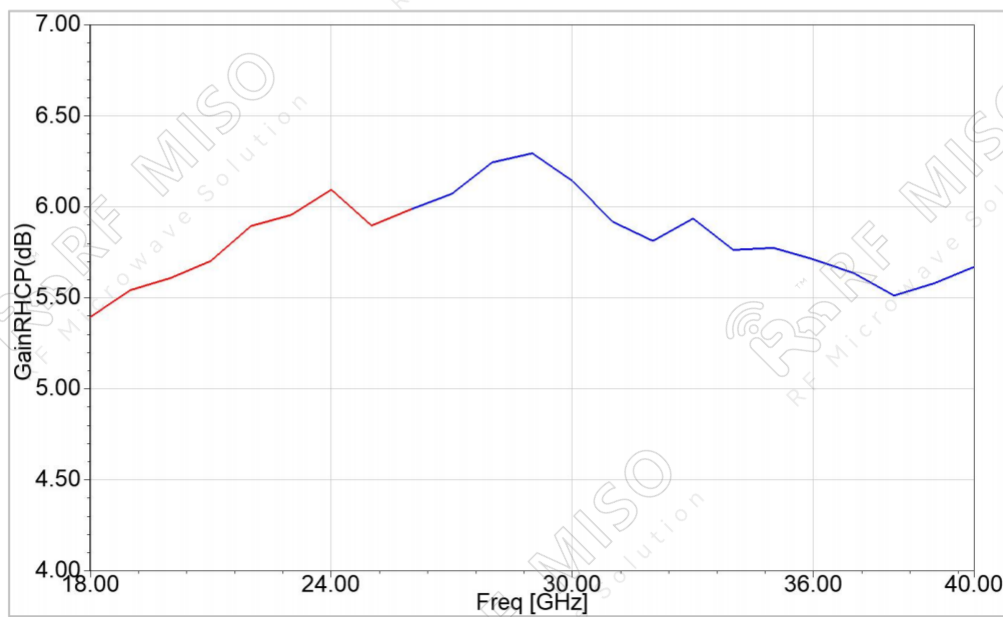
Gain RHCP
