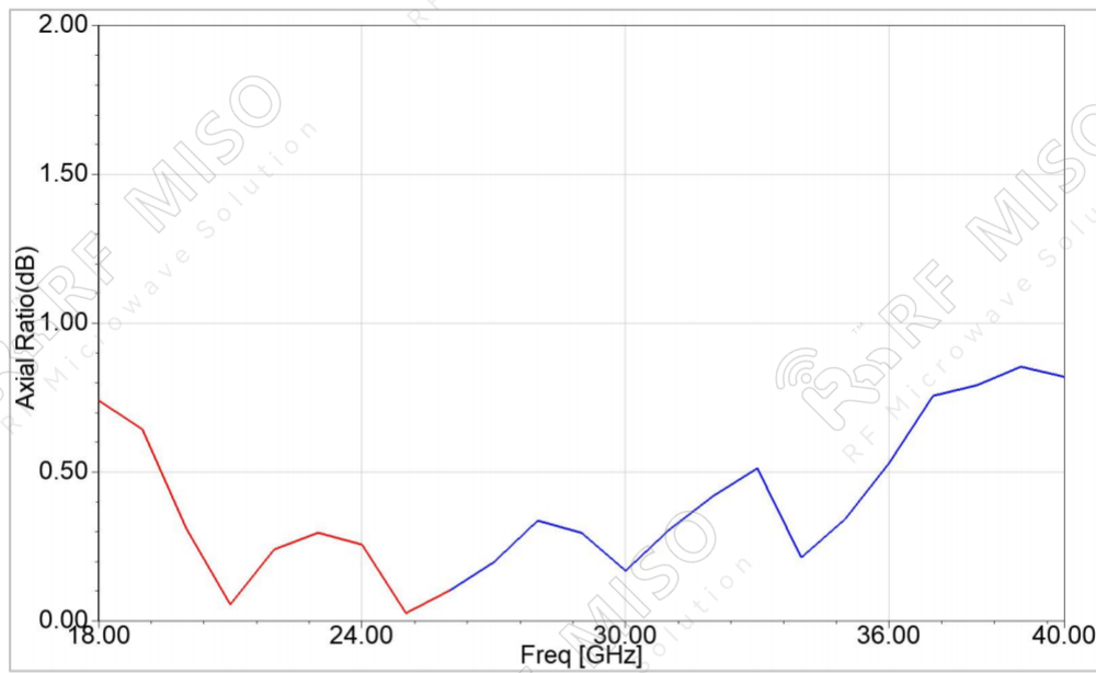
Axial Ratio
