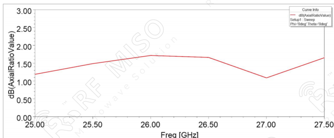
Axial Ratio
