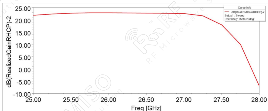
Gain
