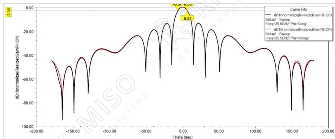
Pattern
