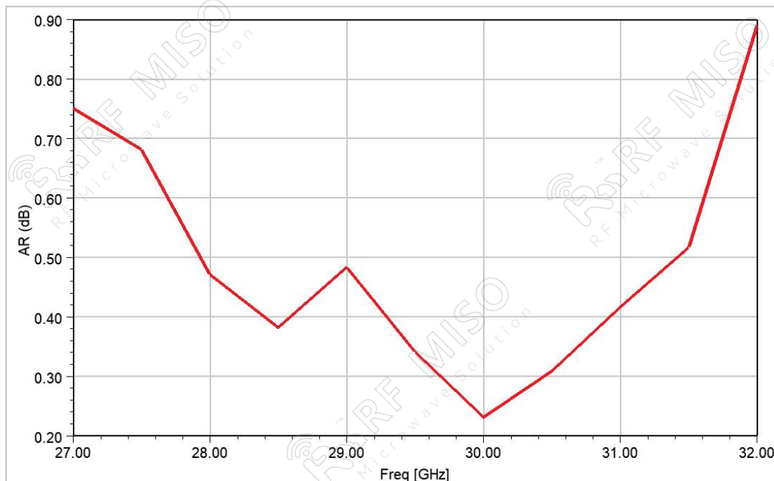
Axial Ratio
