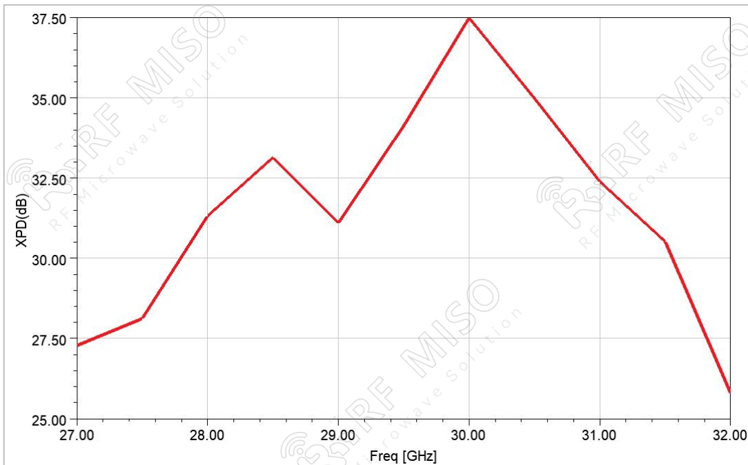
Cross Polarization
