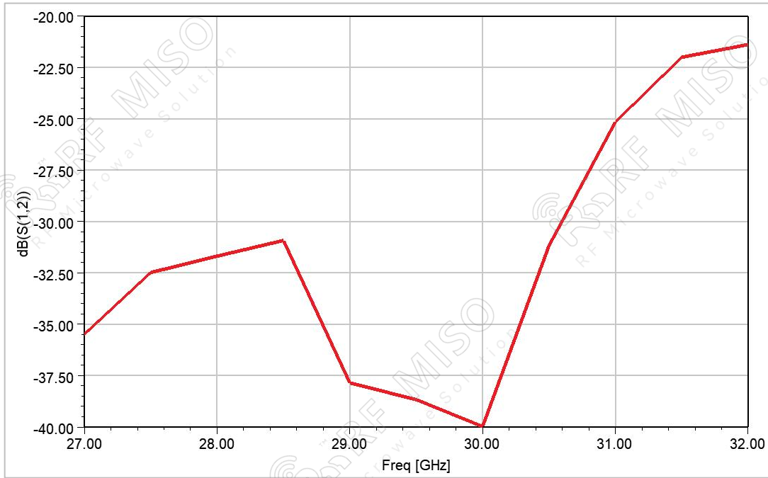
Port-to-port isolation
