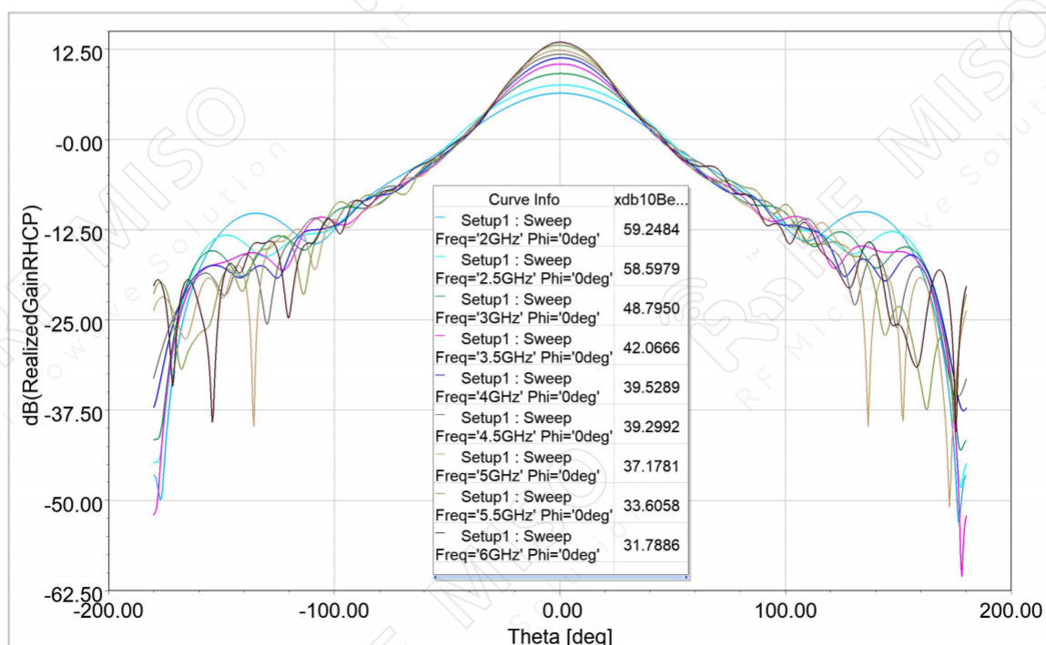
Pattern and 3dB-beamwidth
