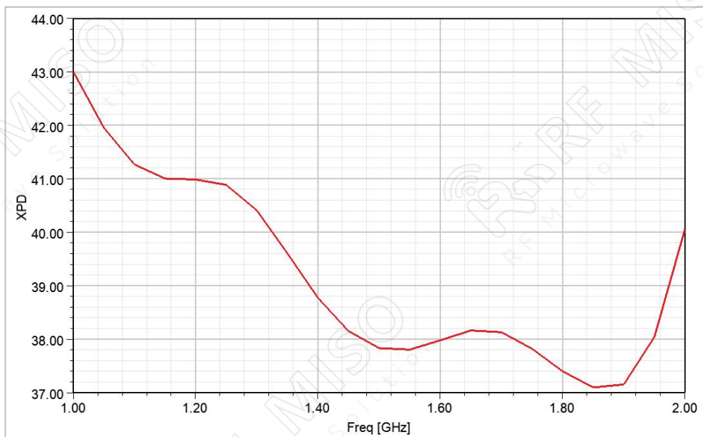
Cross Polarization
