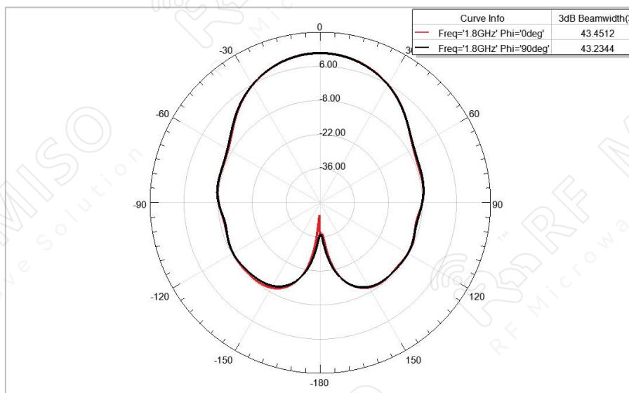
1.8 GHz
