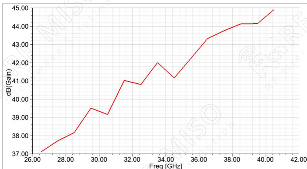
Gain
