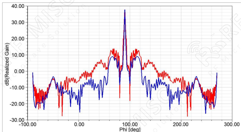
Gain Pattern
