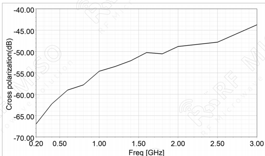
Cross Polarization
