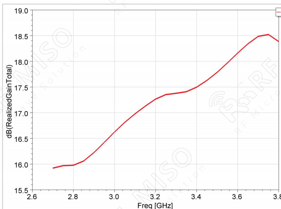
Gain
