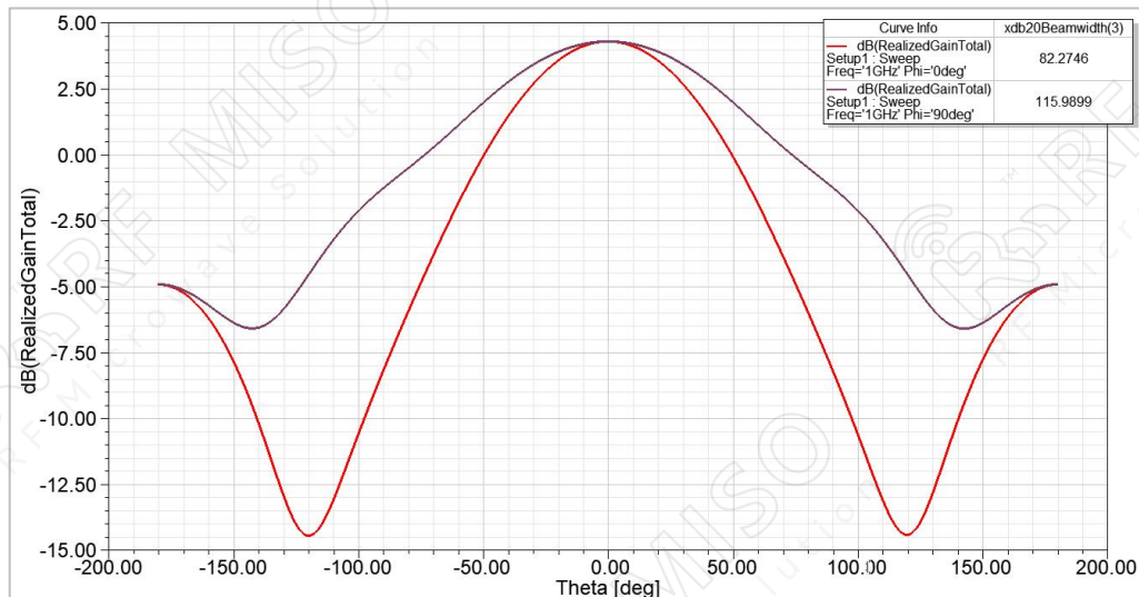
Gain Pattern
